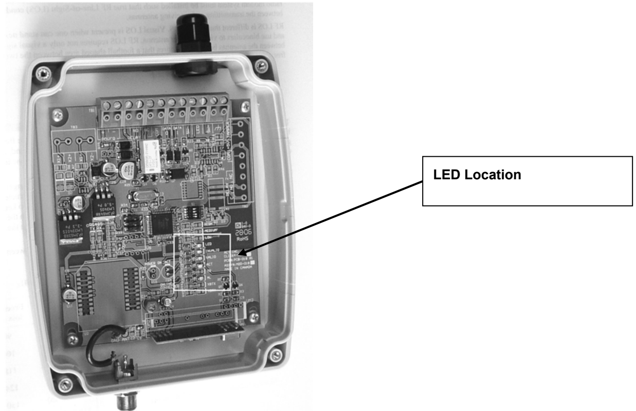
Figure 3 LEDs Location
