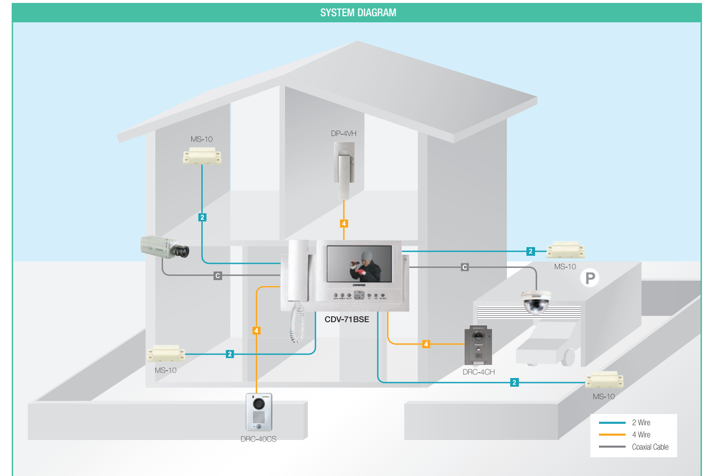
Video Door Phone (Smart View Series)
