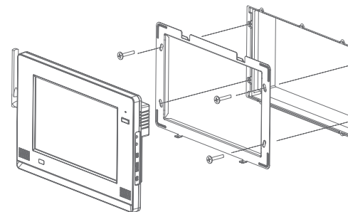
<Mounting diagram>
