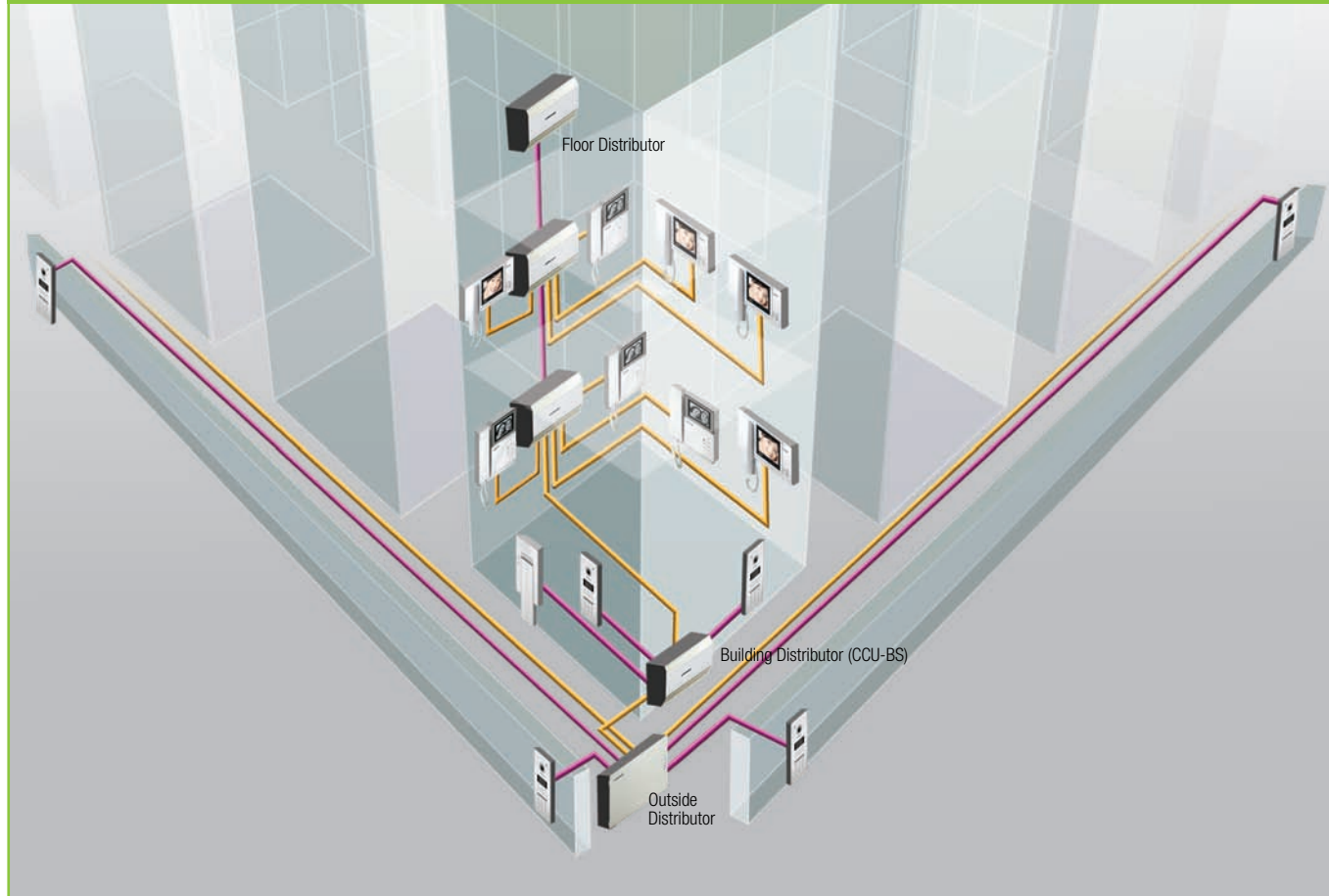
SYSTEM DIAGRAM
