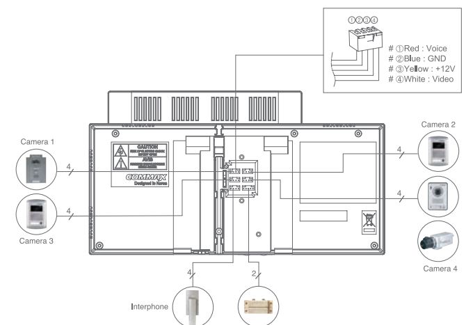
CONNECTING DIAGRAM
