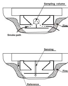
Fig. 1 System schematic
